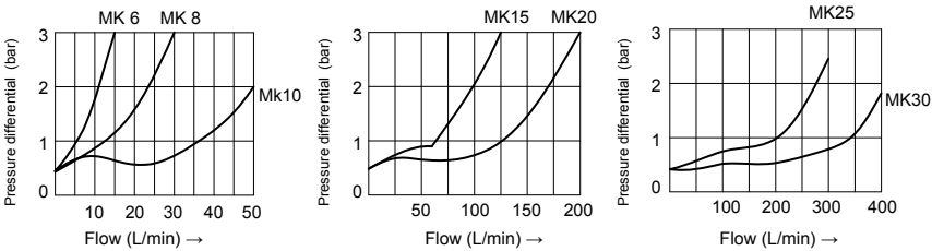
ΔP-Q curves via check valve, with closed throttle (type MK)
