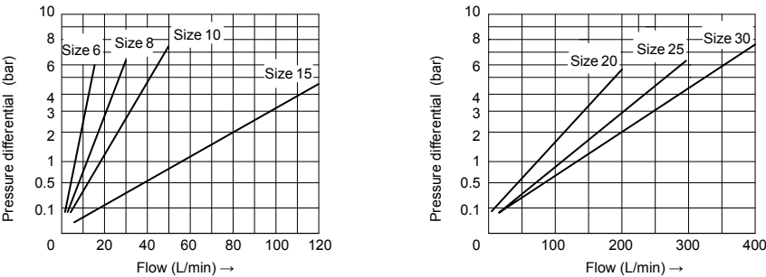
ΔP-Q curves via open throttle (type MG and MK)
