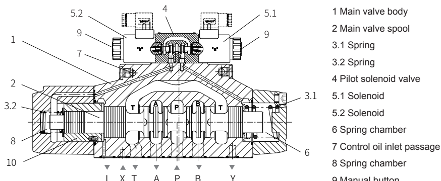
Structure chart of electro-hydraulic directional valves of hydraulic pressure centering
