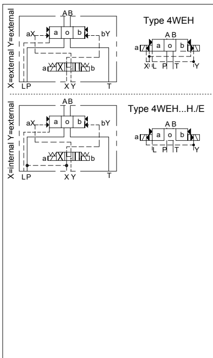
valves with hydraulic centered
