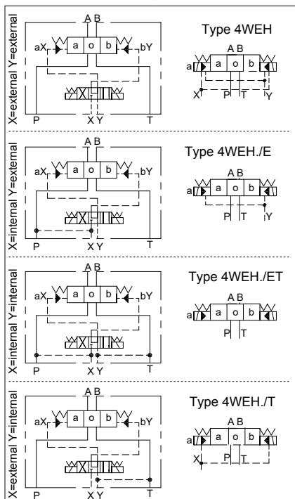
valves with spring centered
