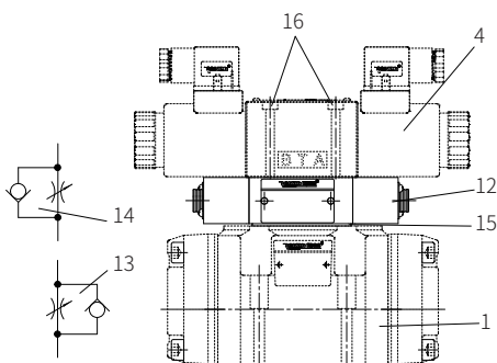
type 4WEH /S or S2
