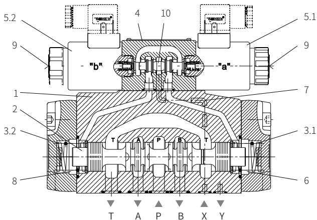
Directional valve Type 4WEH...
